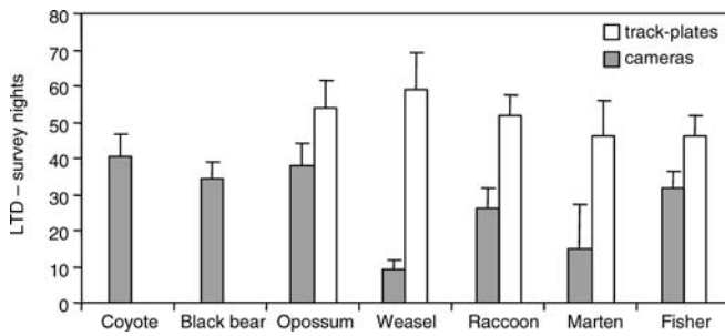
Figure 2. Mean latency to initial detection (LTD) of a species across the Adirondacks during 2000–2002, subdivided by survey technique (cameras and track-plates). Values represent mean lag as measured in number of survey nights \pm SE. Sites are only included if the species was eventually identified at the site by the technique of interest. Note that cameras ran for a greater period (approx. 4 weeks) than track-plates (approx. 2 weeks) at each site, but that fewer ( n = 3 per site) cameras were used than track-plates ( n = 6 per site). Coyotes and black bears were not detected at track-plates.
